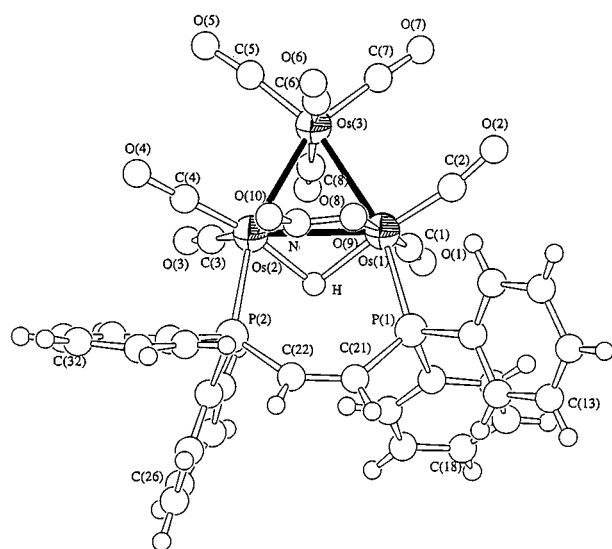
Fig. 5 Molecular structure of [Os 3 (μ-H)(CO) 8 (μ-η 2 -NO 2 )(dppen)] 5a
