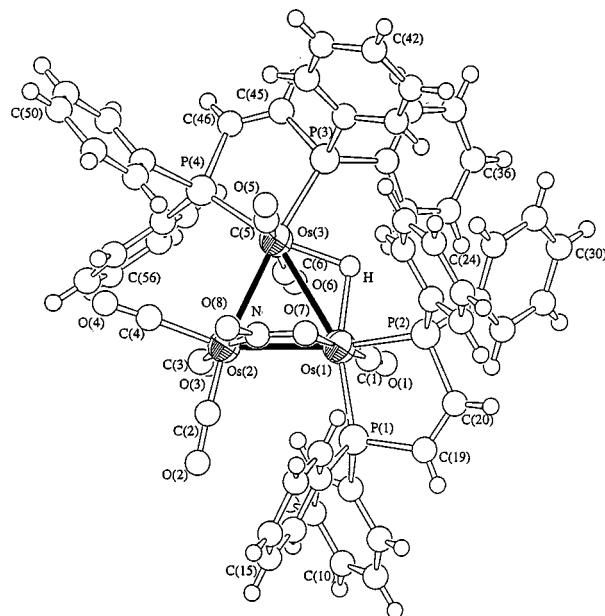
Fig. 6 Molecular structure of [Os 3 (μ-H)(CO) 6 (μ-η 2 -NO 2 )(dppen) 2 ] 6
