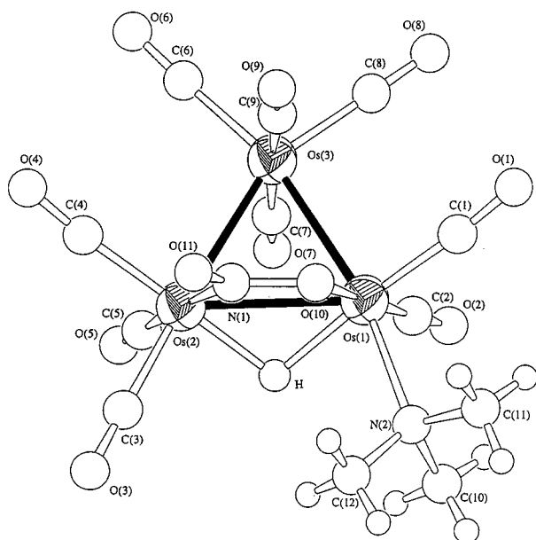
Fig. 1 Molecular structure of [\text{Os}_3(\mu\text{-H})(\text{CO})_9(\mu\text{-}\eta^2\text{-NO}_2)(\text{NMe}_3)] 2a
