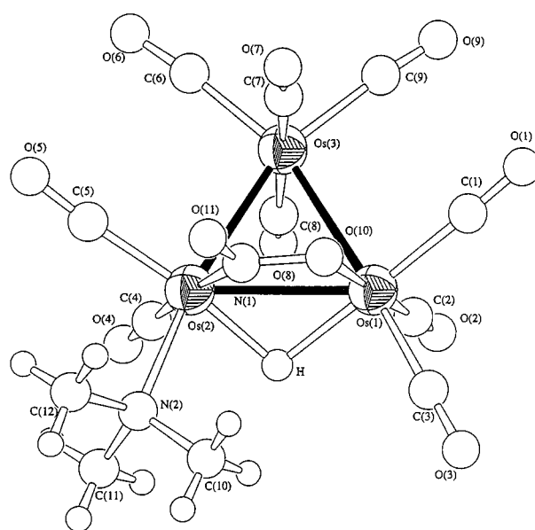
Fig. 2 Molecular structure of [\text{Os}_3(\mu\text{-H})(\text{CO})_9(\mu\text{-}\eta^2\text{-NO}_2)(\text{NMe}_3)] 2b
